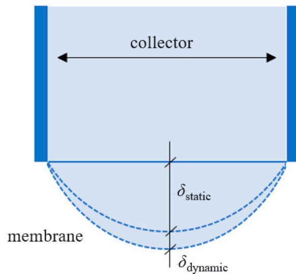
Figure 8. Membrane deformation under static pressure and dynamic pressure.
