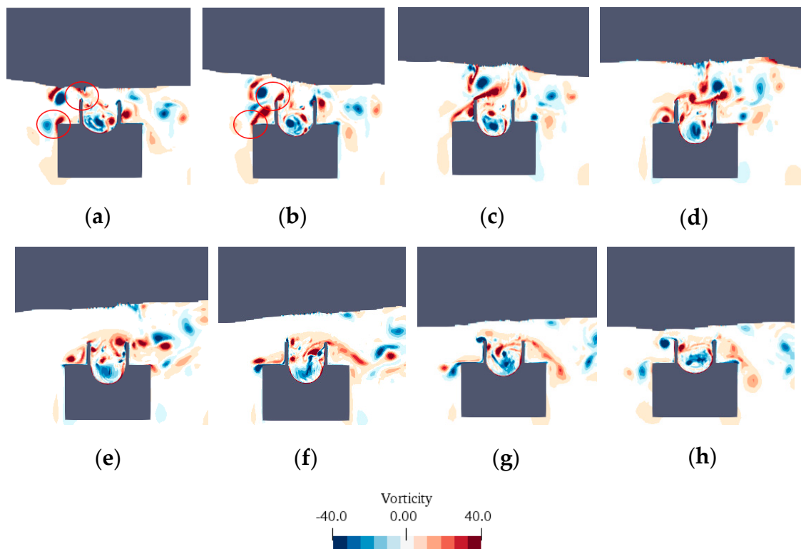
Figure 22. The instantaneous vorticity contour for T = 1.6 s in one wave period ( H = 0.1 m and d = 0.18 m): (a) t = 1/8T , (b) t = 2/8T , (c) t = 3/8T , (d) t = 4/8T , (e) t = 5/8T , (f) t = 6/8T , (g) t = 7/8T , and (h) t = 8/8T .
