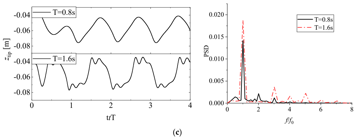
Figure 20. Time histories of the displacement of the membrane tip ( left ) and the FFT results ( right ) with (a) linear-elastic material (b) hyper-elastic M3 (c) hyper-elastic M4 ( H = 0.1 m and d = 0.18 m for T = 0.8 s and 1.6 s).
